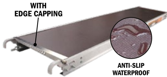
ALUMINUM PLATFORM WITH 5/8" ANTI-SLIP PLYWOOD DECK WITH EDGE CAPPING
